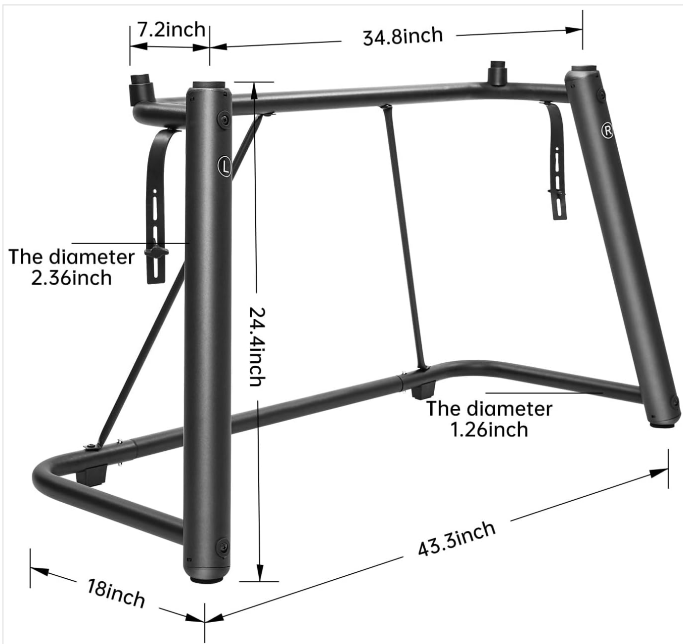
Figure 6: Detailed dimensions of the AODSK U-Shaped Keyboard Display Stand, including height, width, and depth measurements.
