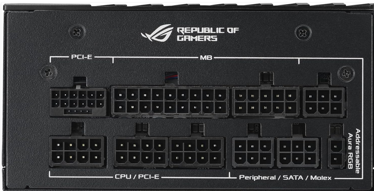
Figure 3: Modular cable connection ports on the power supply, labeled for PCI-E, MB (Motherboard), CPU/PCI-E, and Peripheral/SATA/Molex connections, including an Addressable Aura RGB header.
