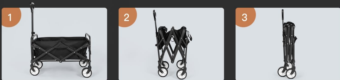
Figure 5.1: The wagon's compact folded dimensions (25.6" x 18.0" x 5.1") for easy storage.
