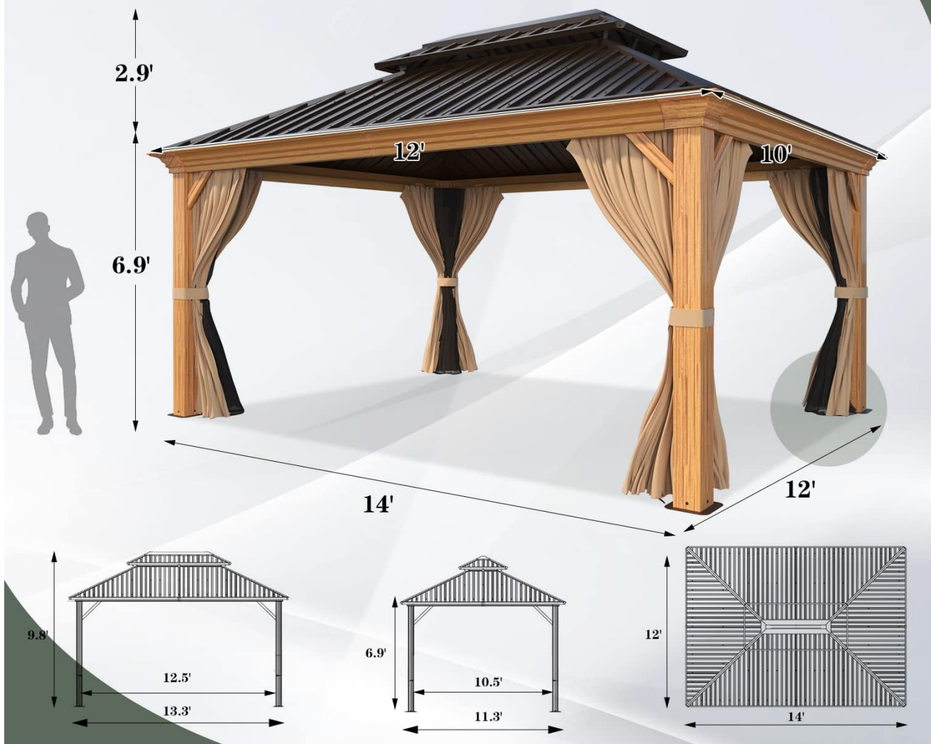
Image: Detailed diagram of all gazebo components and their quantities, including overall dimensions.
