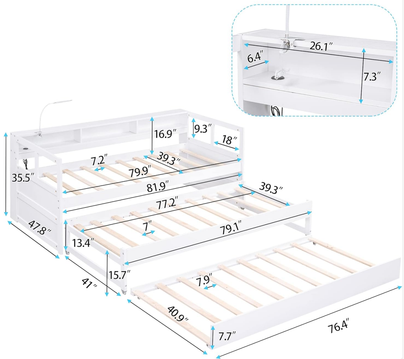
Image 4.1: Dimensional diagram of the Polibi Twin XL Daybed, including the main bed, trundles, and storage cubbies. Refer to this for space planning.
