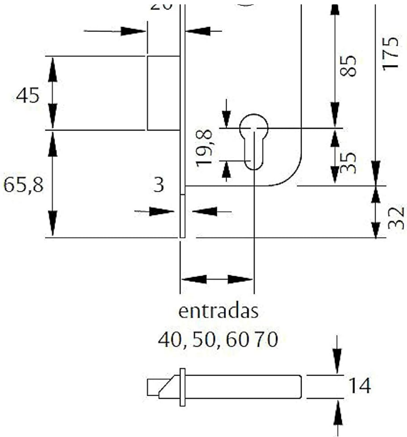
Figure 3: Technical dimensions of the Tesa Assa Abloy Mortise Lock. This diagram provides critical measurements such as backset (Entrada), axle spacing (85 mm), and overall lock body dimensions, essential for accurate door preparation and installation.
