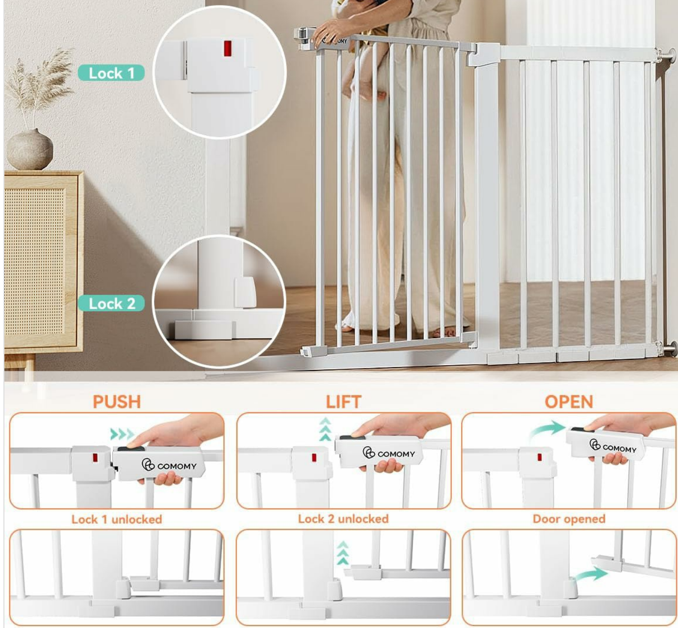
Figure 7: Dual Locking Mechanism for secure operation.
