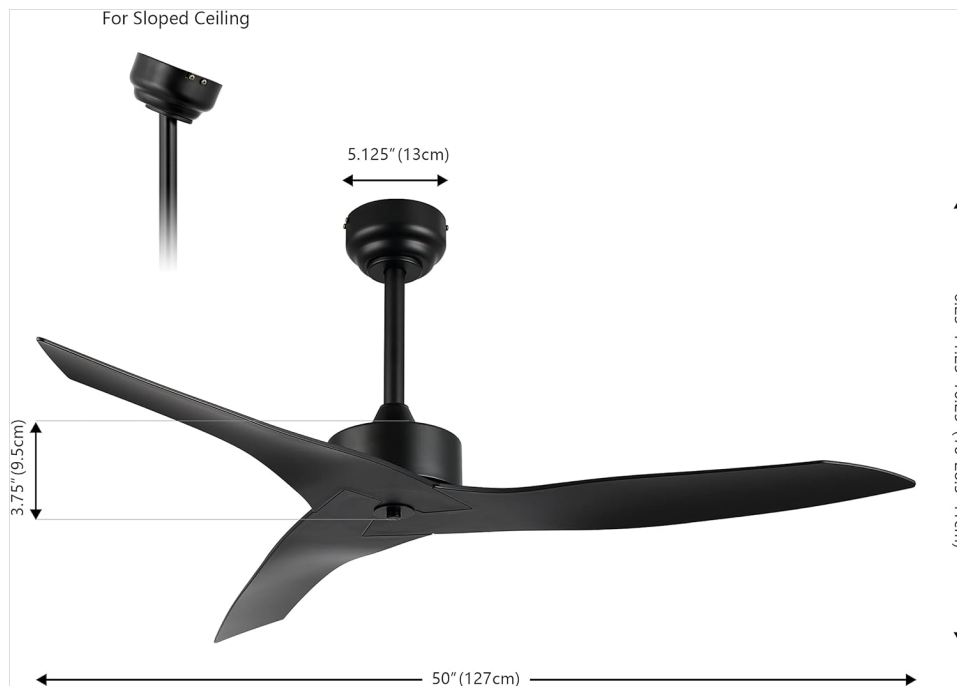
Image: Technical drawing illustrating the fan's dimensions, including overall width (50 inches) and various height options (6.25 to 16.25 inches).
