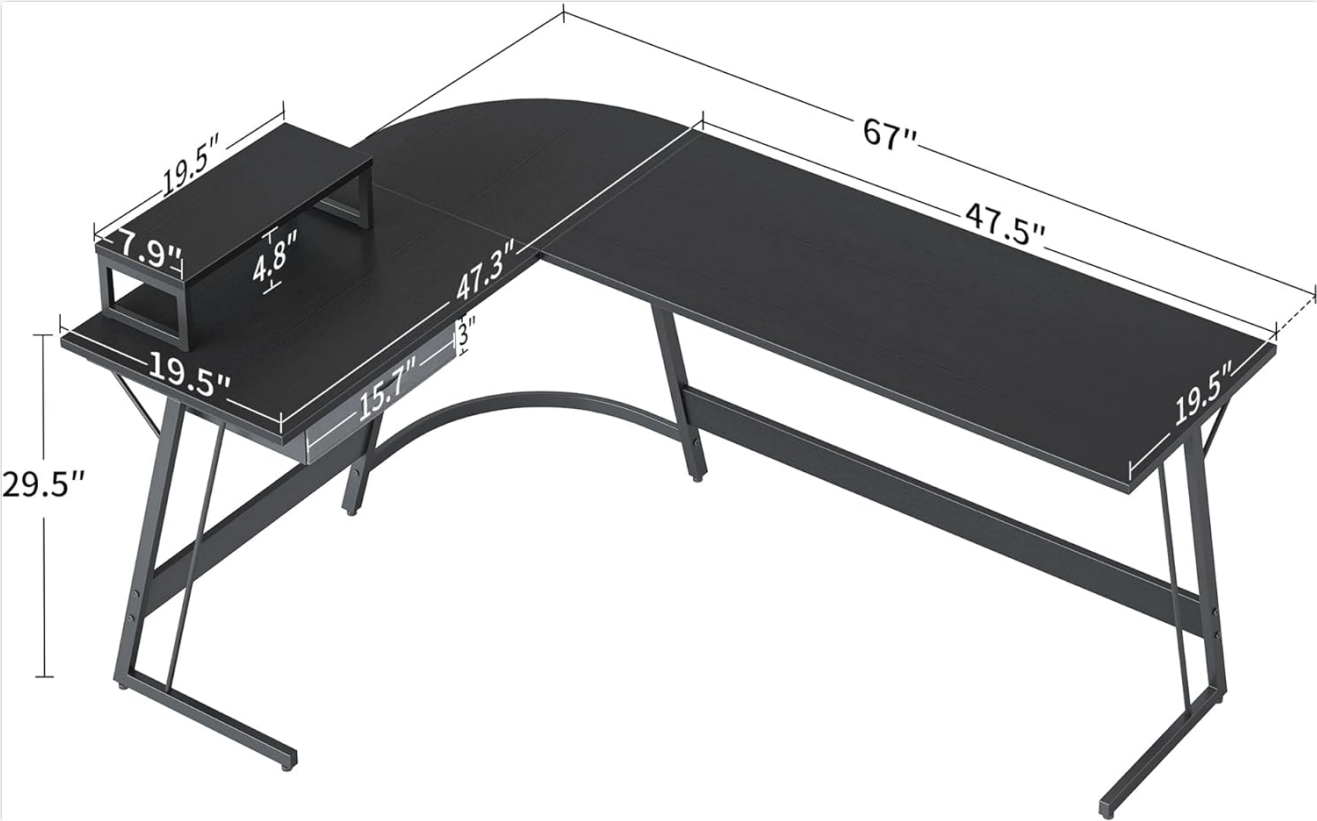
Figure 8.1: Key dimensions of the BANTI 67-inch L-Shaped Desk.
