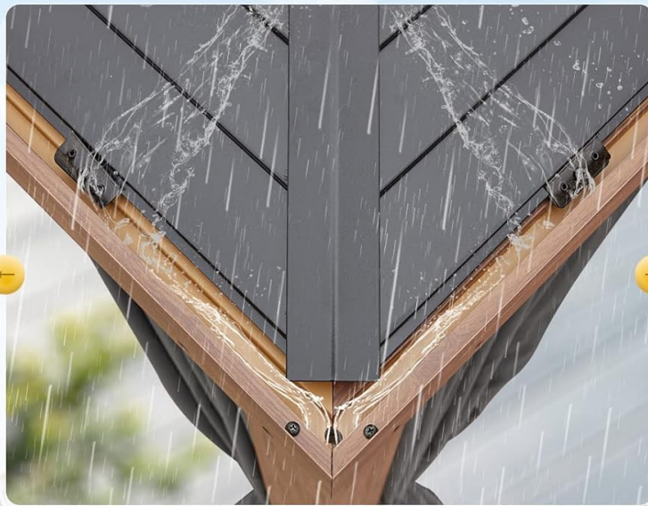
Figure 3: Double-top roof design with ventilation and drainage features.
