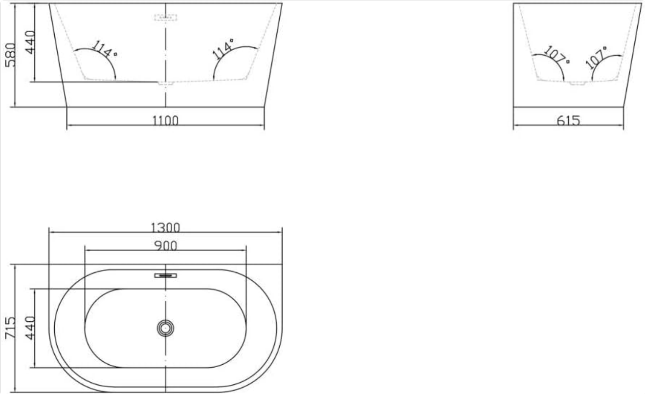
Image: Technical drawing showing the length (130cm), width (71.5cm), and height (58cm) of the DIVINA bathtub, along with internal dimensions and angles for installation planning.
