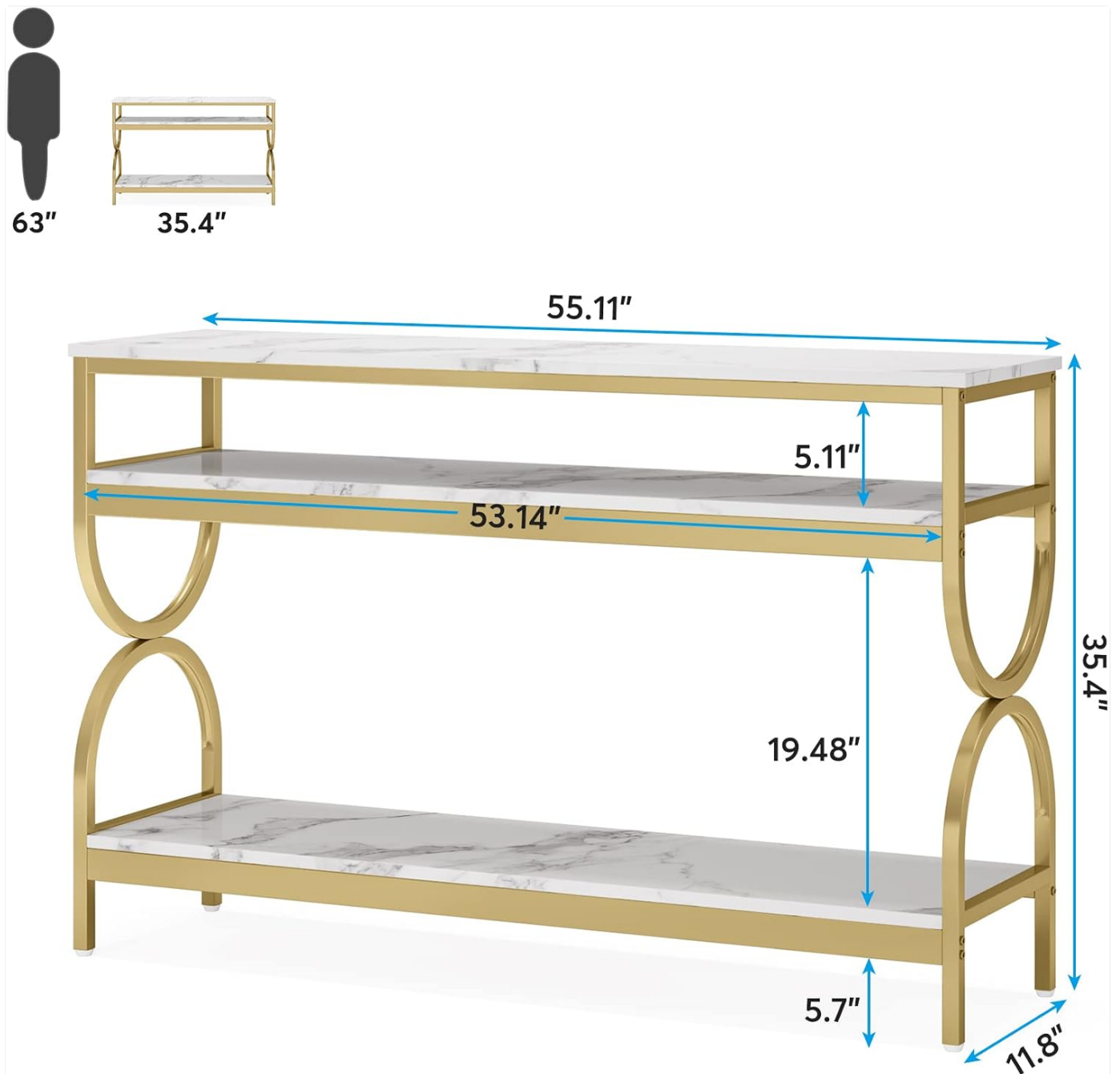
Figure 4.1: Product Dimensions. This diagram illustrates the key dimensions of the console table: 55.11 inches in width, 11.8 inches in depth, and 35.4 inches in height. It also shows the spacing between the shelves.
