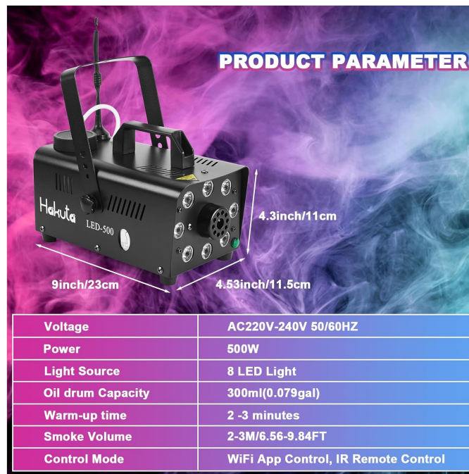
Image: A table detailing the technical specifications of the Hakuta LED-500 Fog Machine.
