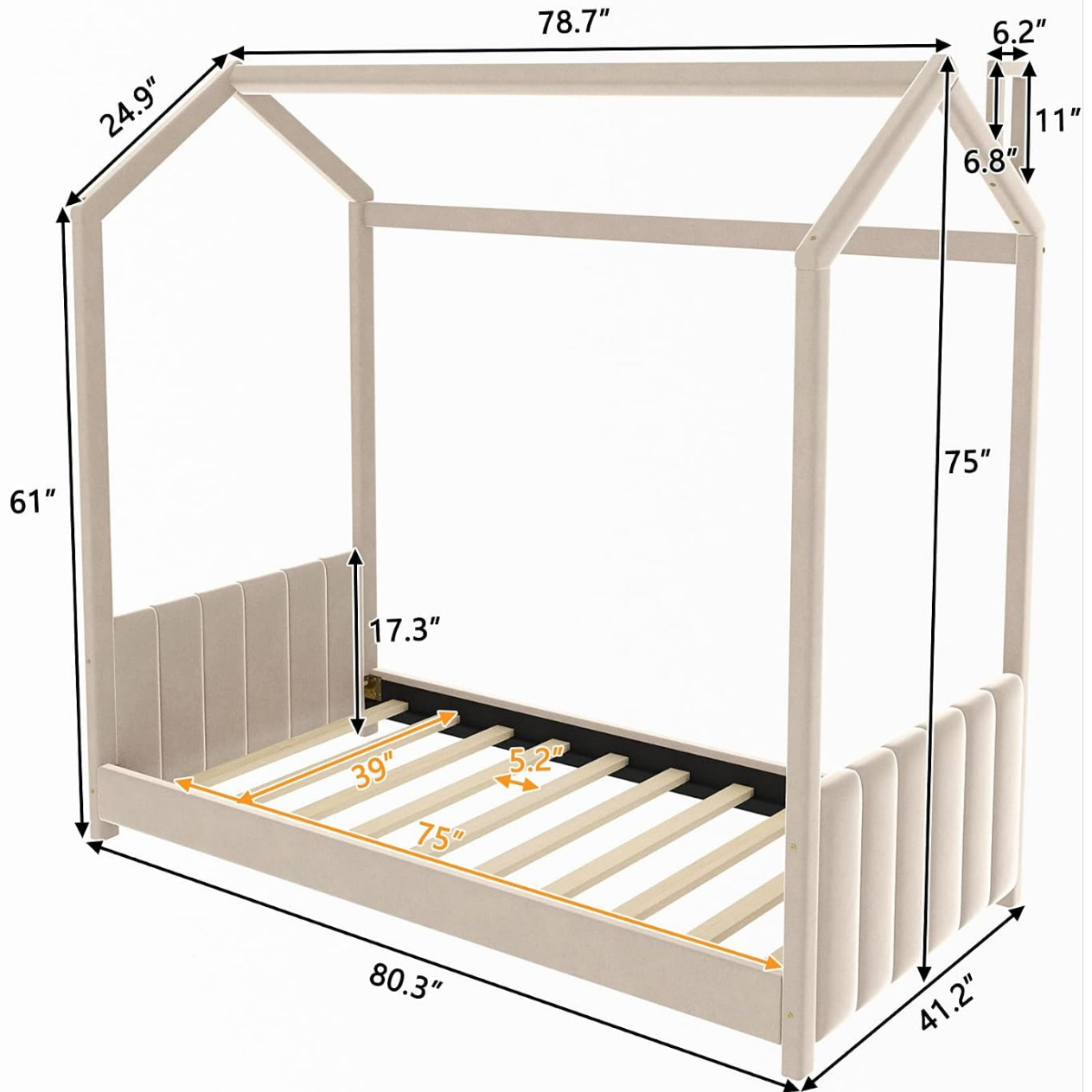
Image: Dimensional drawing of the bed frame, showing length, width, and height measurements.
