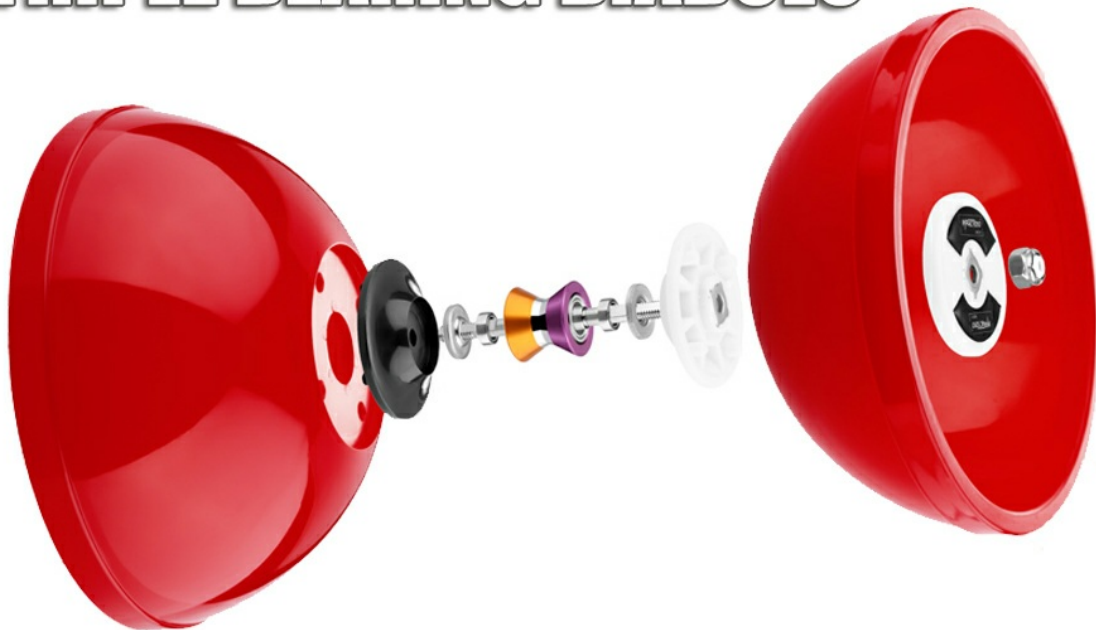
Image: Internal structure of the MD01 Pro Diabolo, highlighting the triple bearing design.
