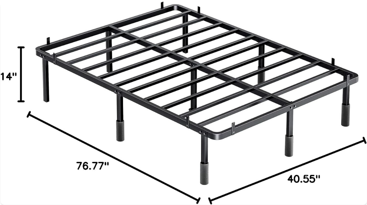
Diagram showing the dimensions of the Marsail MSBFT01 Twin size bed frame: 76.77 inches length, 40.55 inches width, and 14 inches height.
