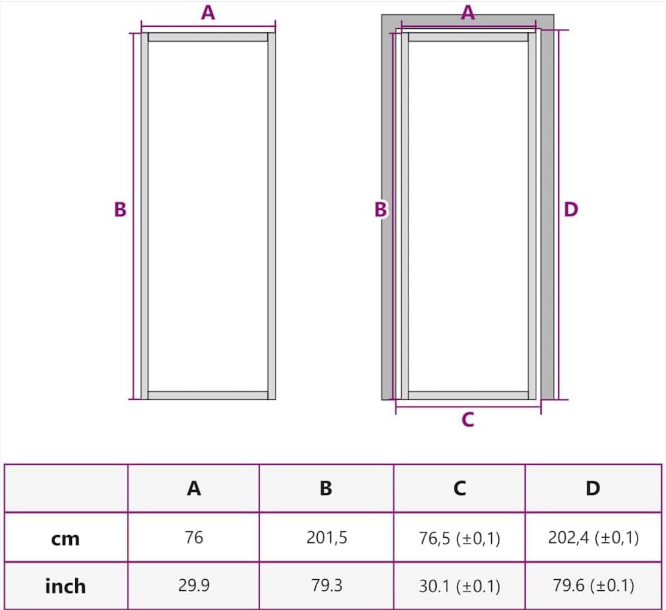
Image 4.1: Installation dimensions. A: 76 cm (29.9 inches), B: 201.5 cm (79.3 inches), C: 76.5 cm (30.1 inches), D: 202.4 cm (79.6 inches).
