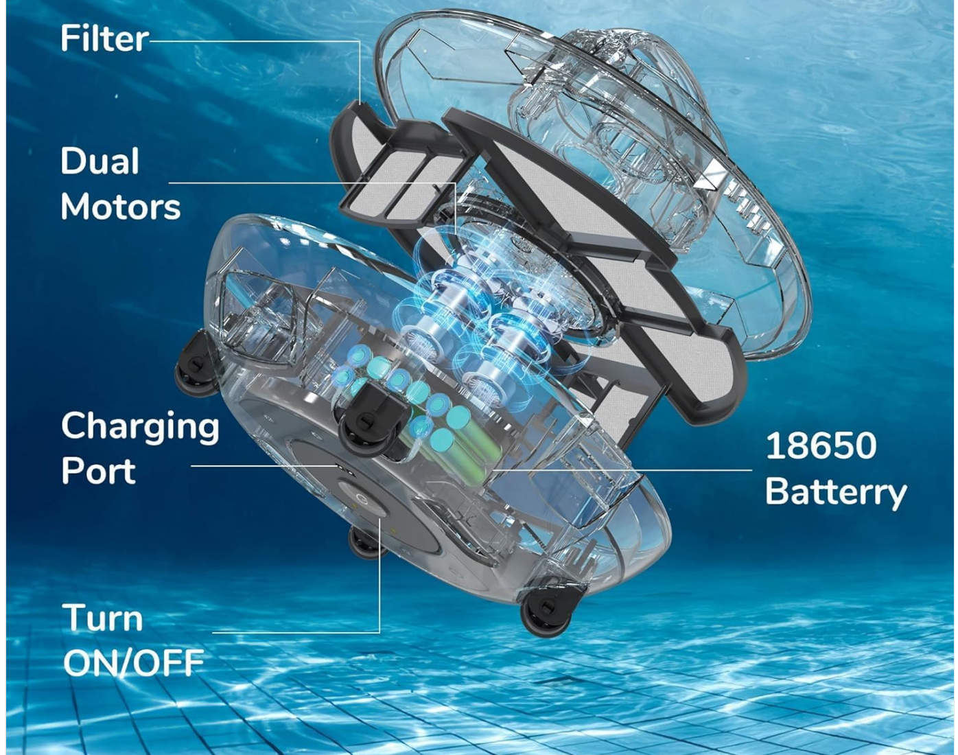
Image: An exploded view diagram of the G900 cleaner, highlighting key internal components such as the filter, dual motors, charging port, and the ON/OFF switch.
