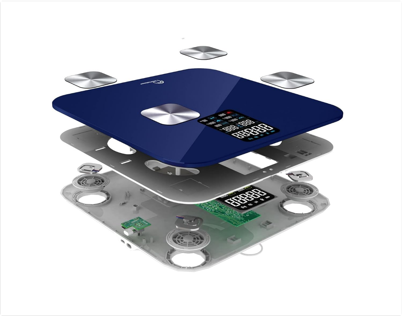
Image: An exploded view of the scale, illustrating its internal components and modular design for repairability.
