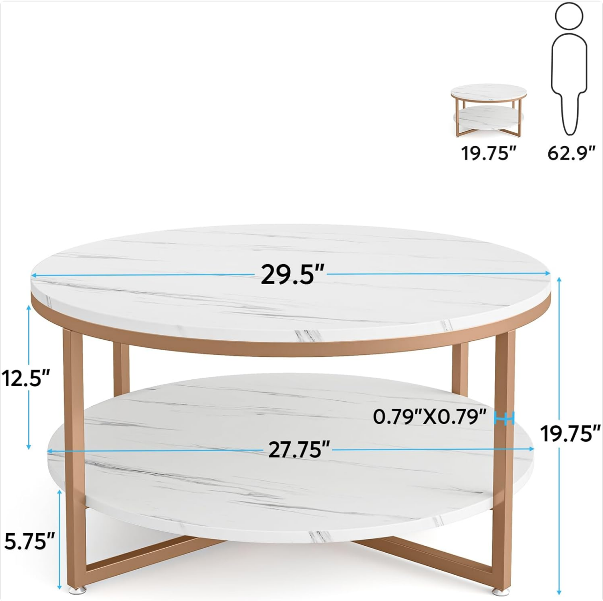
Image 6.1: Dimensional diagram of the coffee table.
