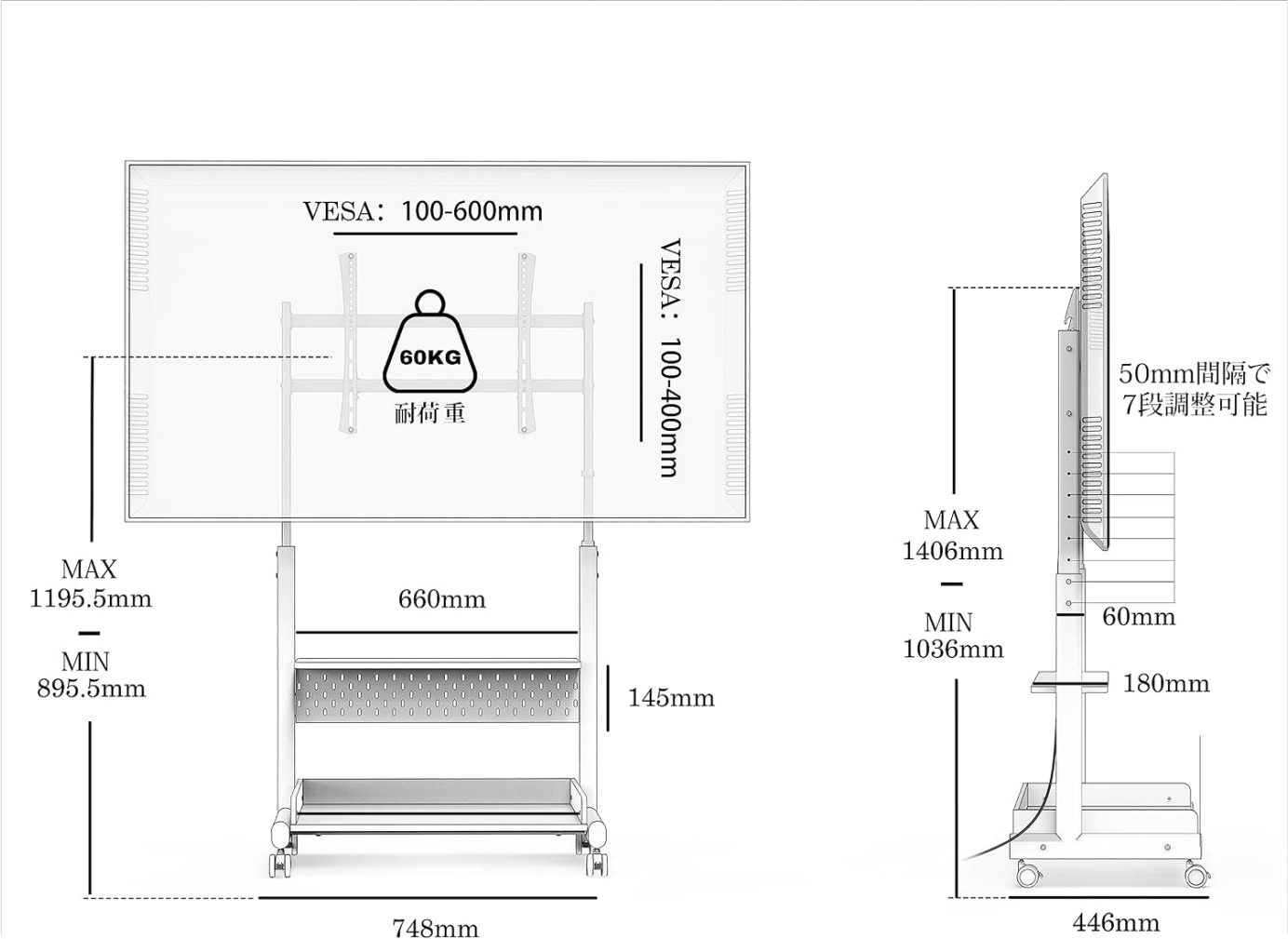
Detailed dimensions and VESA mounting specifications.
