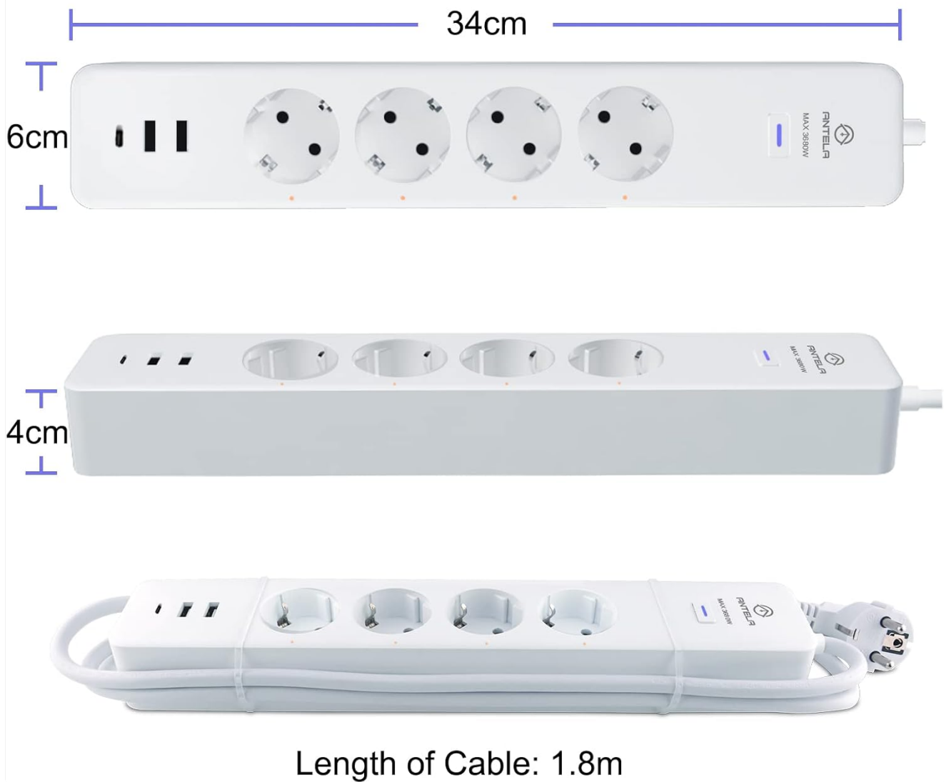
Figure 2.2: Physical dimensions of the power strip. The device measures 34cm in length, 6cm in width, and 4cm in height. The attached power cable is 1.8 meters long.
