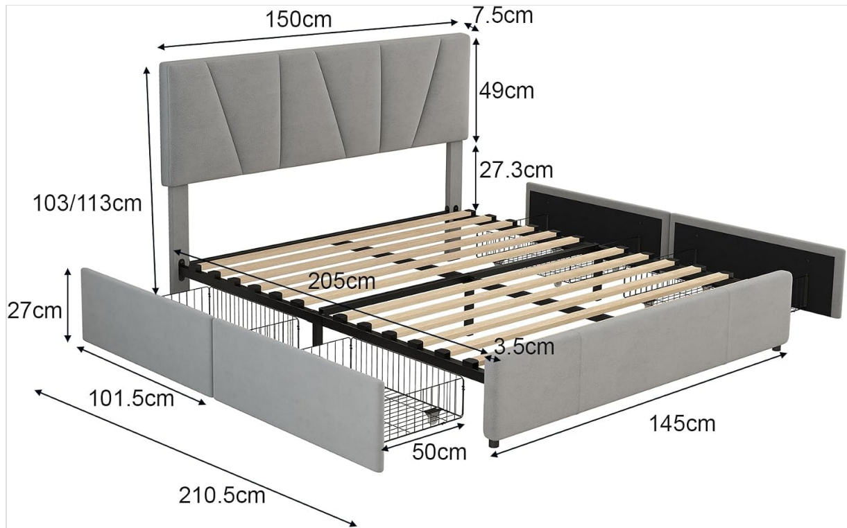
Image: Detailed dimension diagram of the ModernLuxe bed frame, showing all key measurements.
