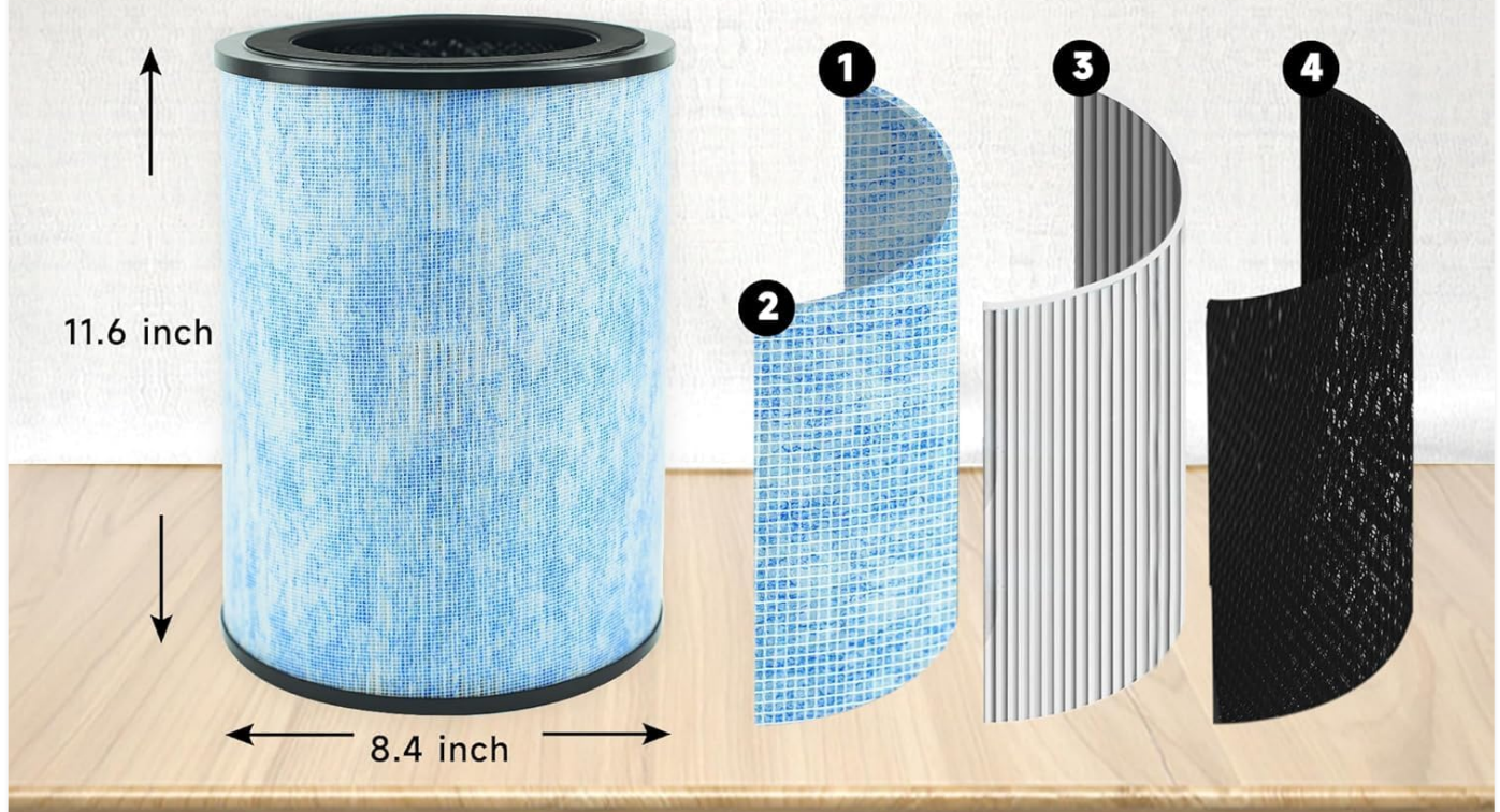
Image 2: Detailed view of the 3-in-1 filtration layers.
