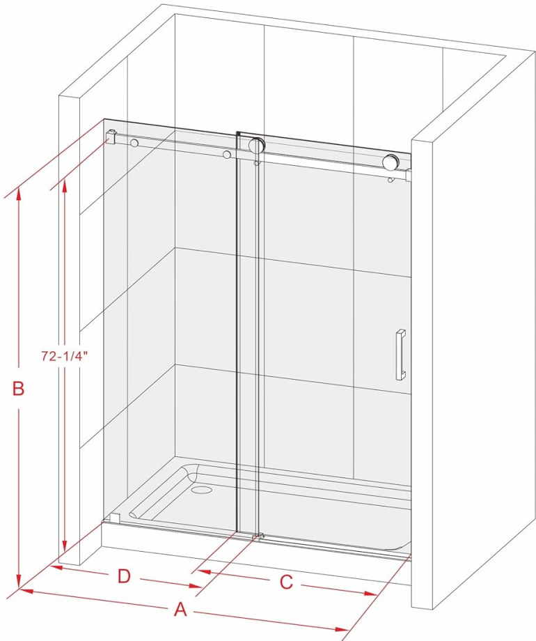
Image: Diagram illustrating the overall dimensions of the UKS05-5576-CH shower door, including model width, height, door width, and fixed panel dimensions.
