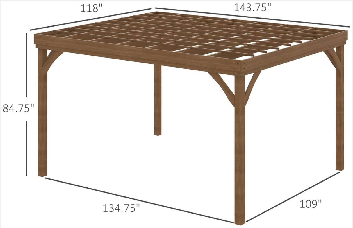
Figure 5: Product dimensions.
