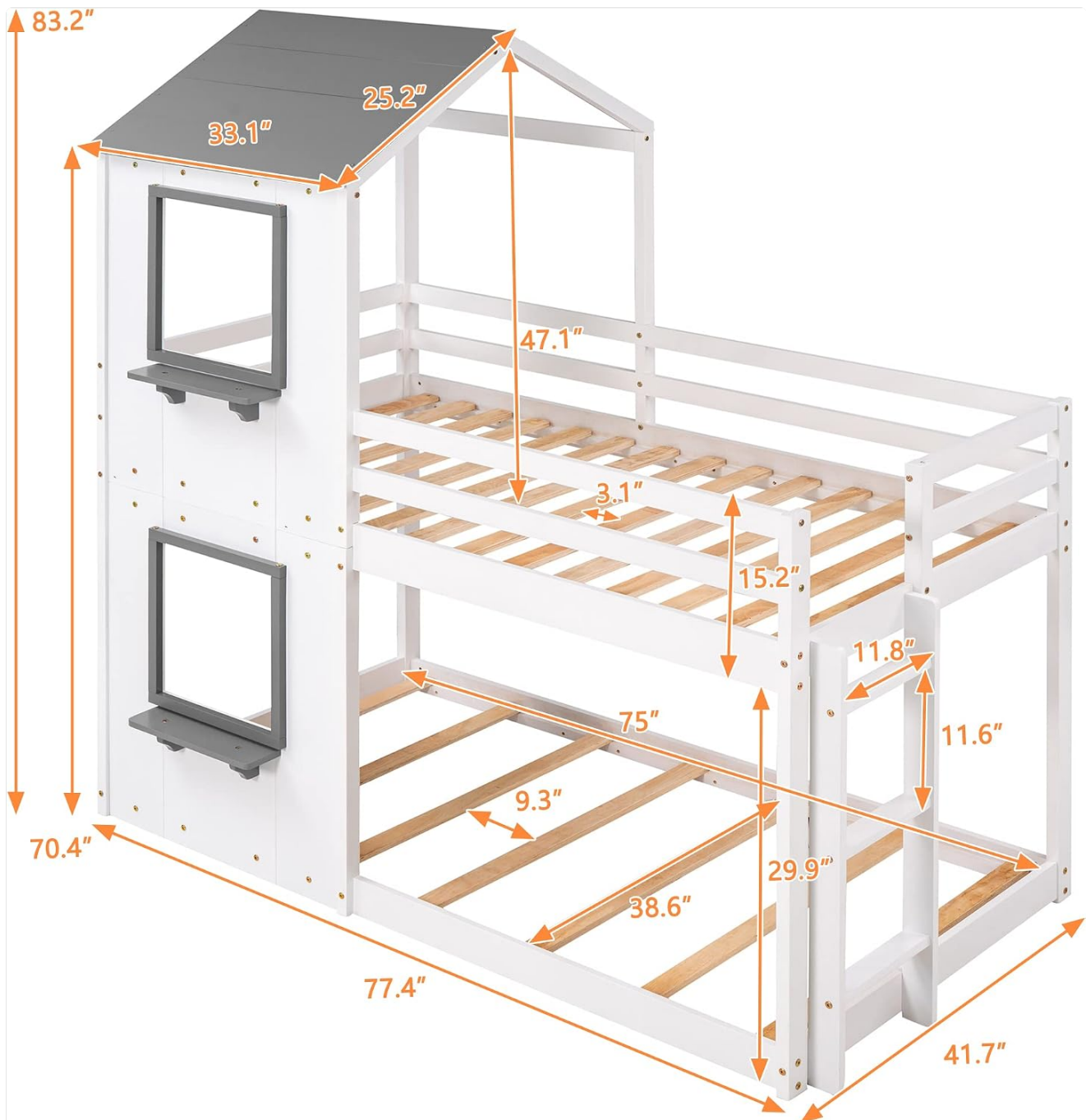
Figure 2: Detailed dimensions of the bunk bed, including length, width, height, and spacing between bunks.
