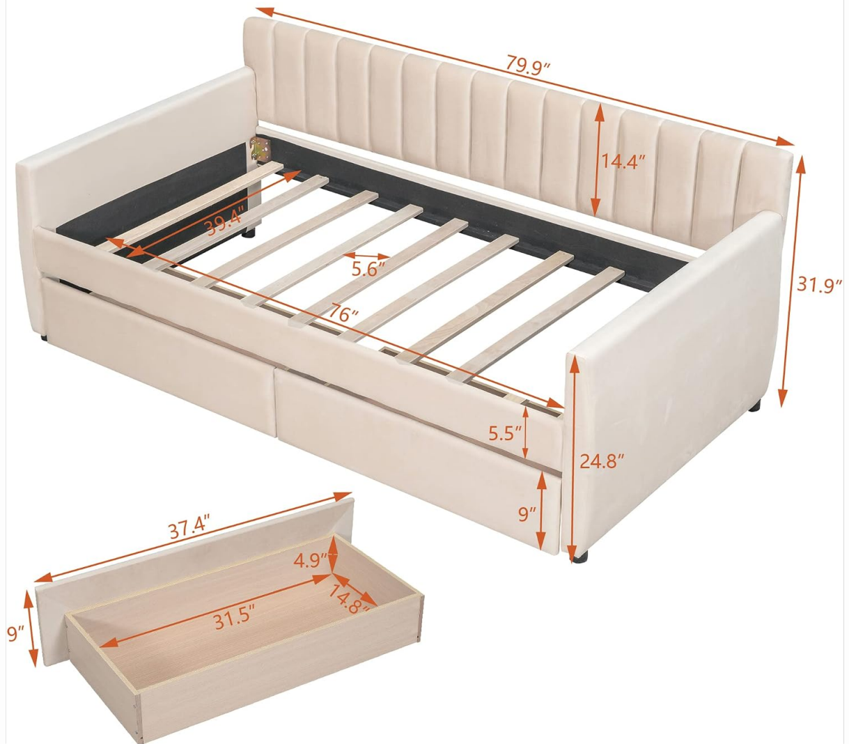
Image: Detailed dimensions of the daybed, including overall length, width, height, and drawer measurements.
