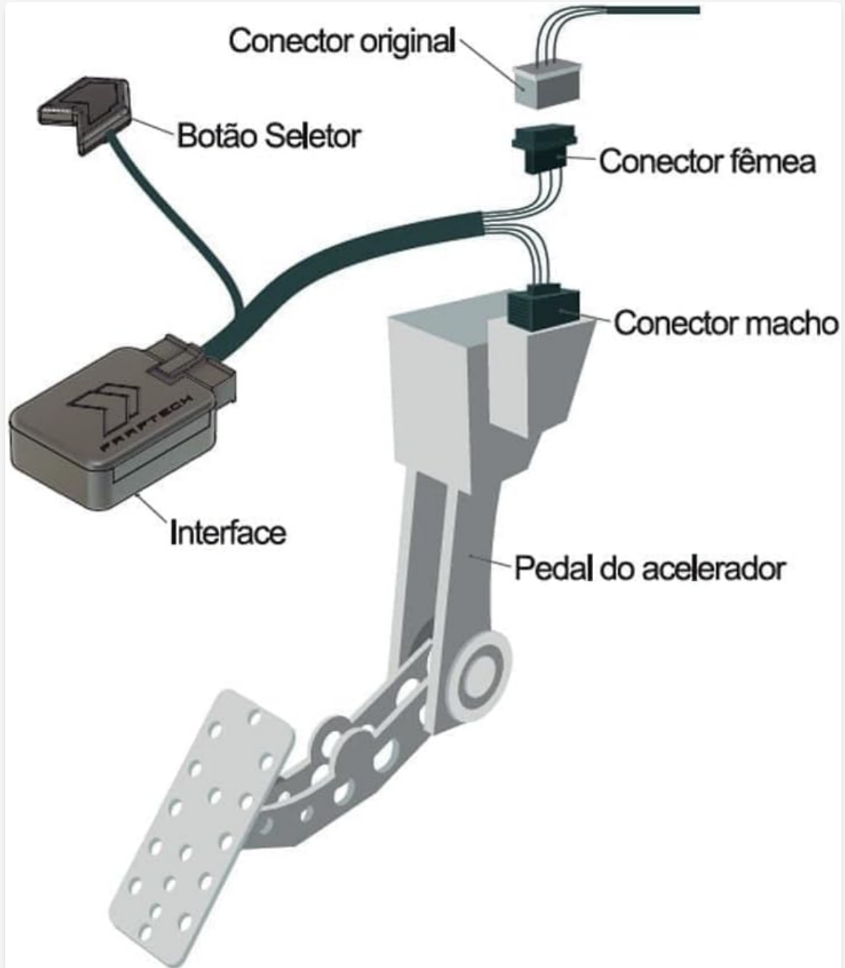
Image 3.1: Installation diagram illustrating the connection of the Shiftpower interface, toggle button, and harness to the vehicle's accelerator pedal.
