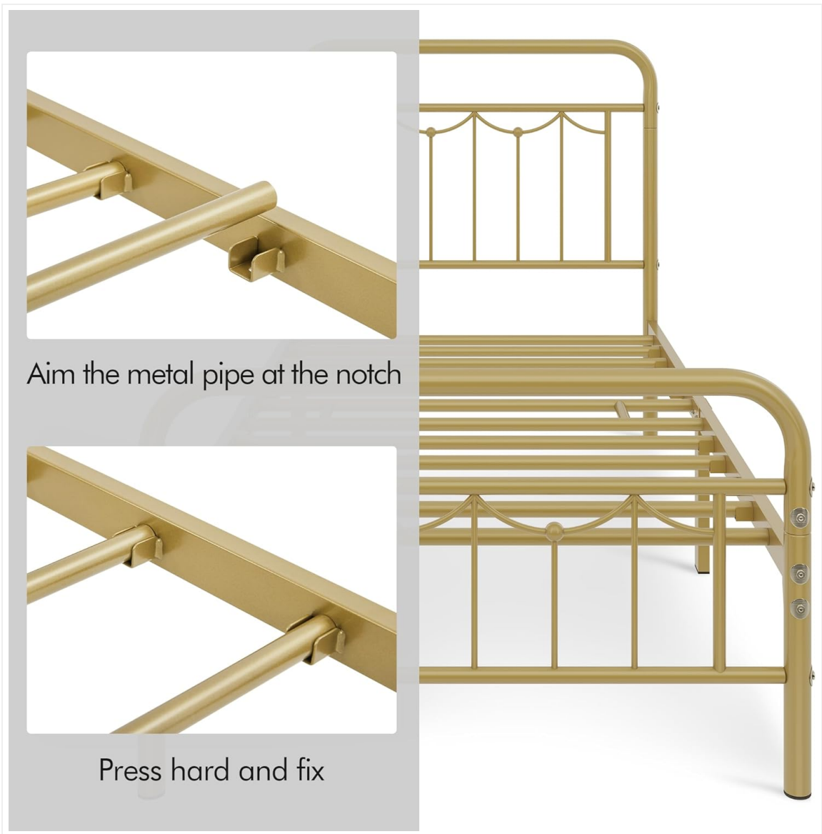
Image: Illustration demonstrating how to aim the metal pipe at the notch and press to secure the slats.
