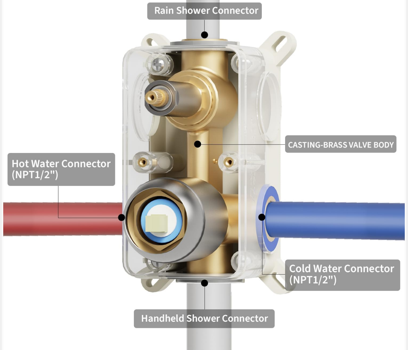
Figure 2: Brass Shower Valve Connections. This diagram illustrates the internal structure and connection points of the valve.
