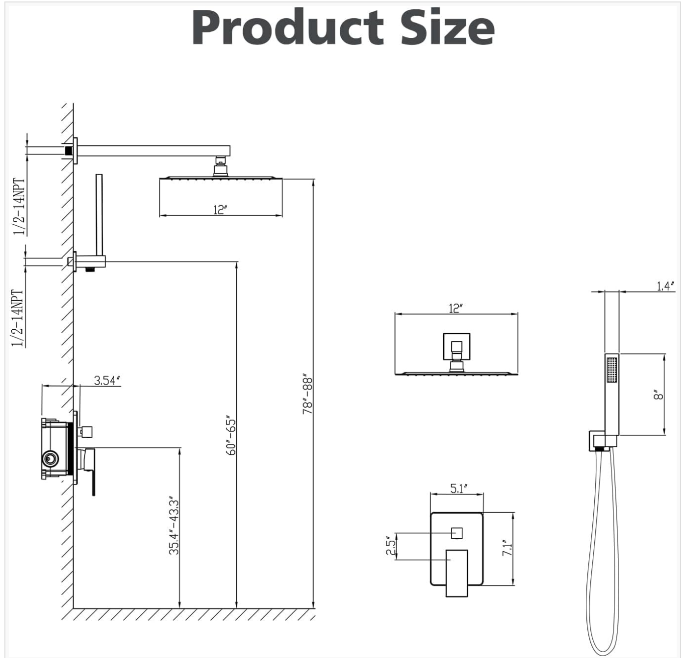
Figure 1: Product Dimensions. Refer to this diagram for precise measurements and rough-in specifications.
