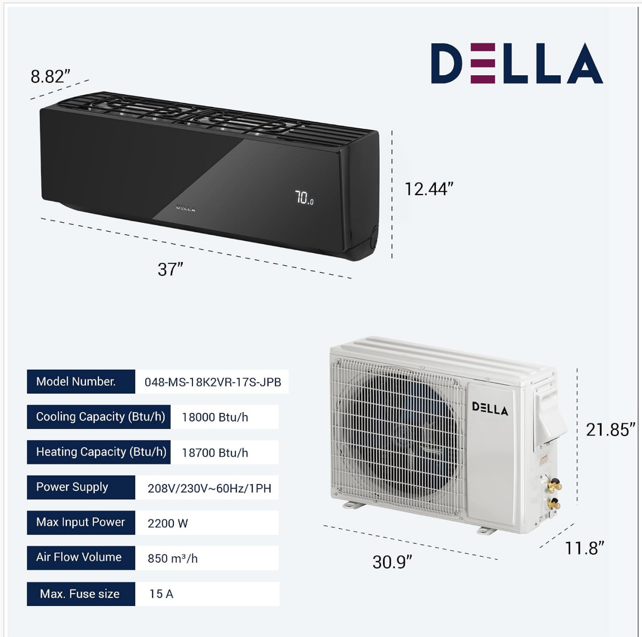
Figure 8.1: Dimensions of the indoor and outdoor units.
