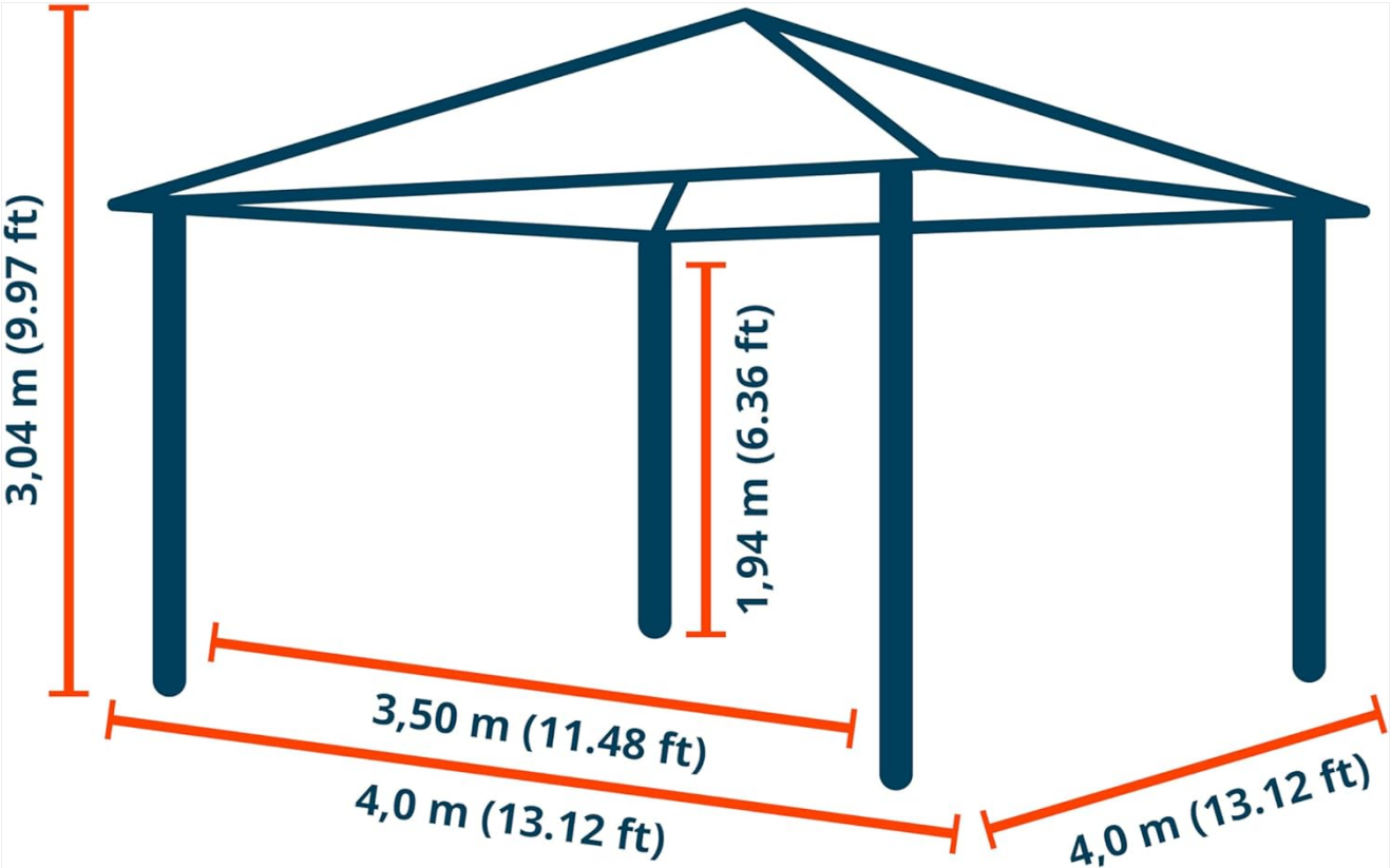
Image 9: Dimensional diagram of the gazebo, indicating its length, width, and height for planning purposes.
