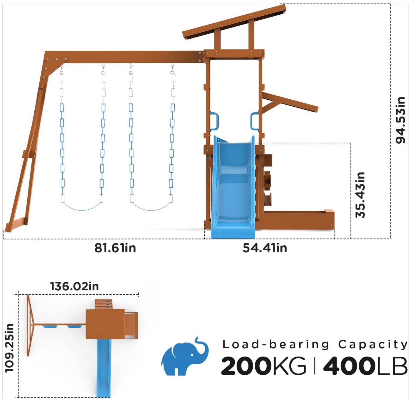
Figure 9.1: Detailed dimensions of the DOLPHIN PLAYGROUND T Wooden Swing Set.
