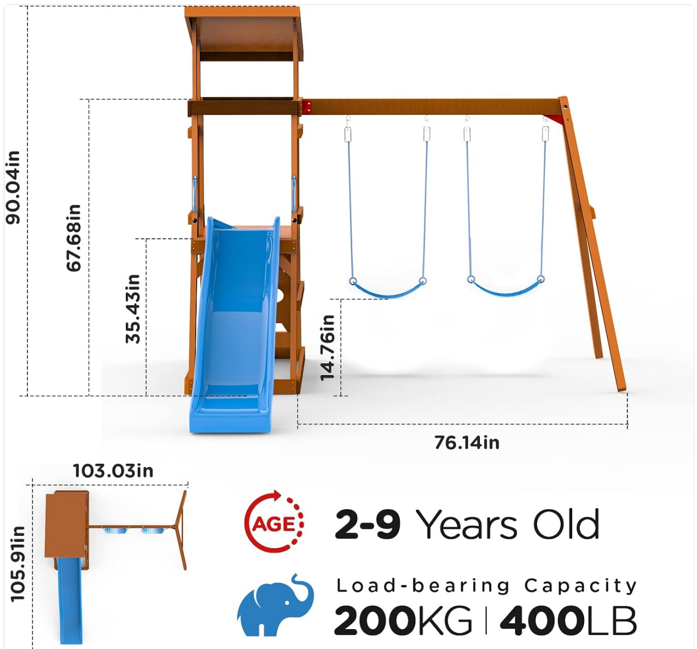
Figure 3.2: Playset Dimensions. A detailed diagram illustrating the overall dimensions of the swing set, including the height of the fort, the length of the swing beam, and the footprint of the entire structure.
