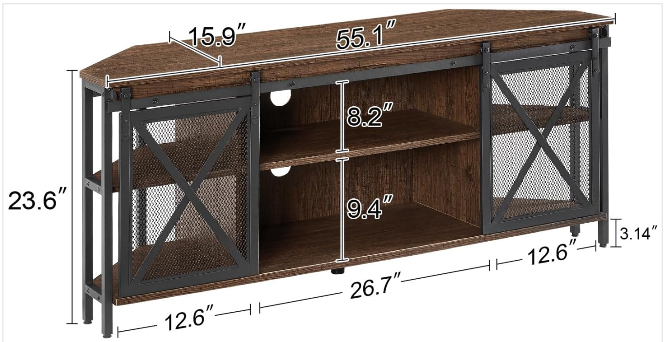
Figure 1: Product Dimensions. This image illustrates the overall dimensions of the TV stand, including its length (55.1 inches), depth (15.9 inches), and height (23.6 inches), along with shelf heights.
