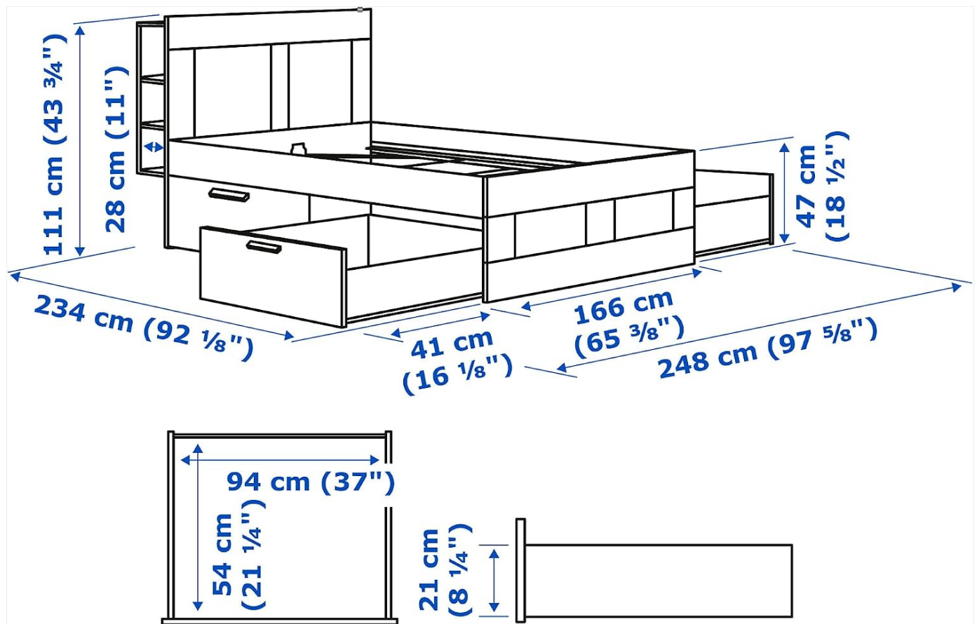
Figure 3: Dimensional drawing of the BRIMNES bed frame, indicating key measurements.
