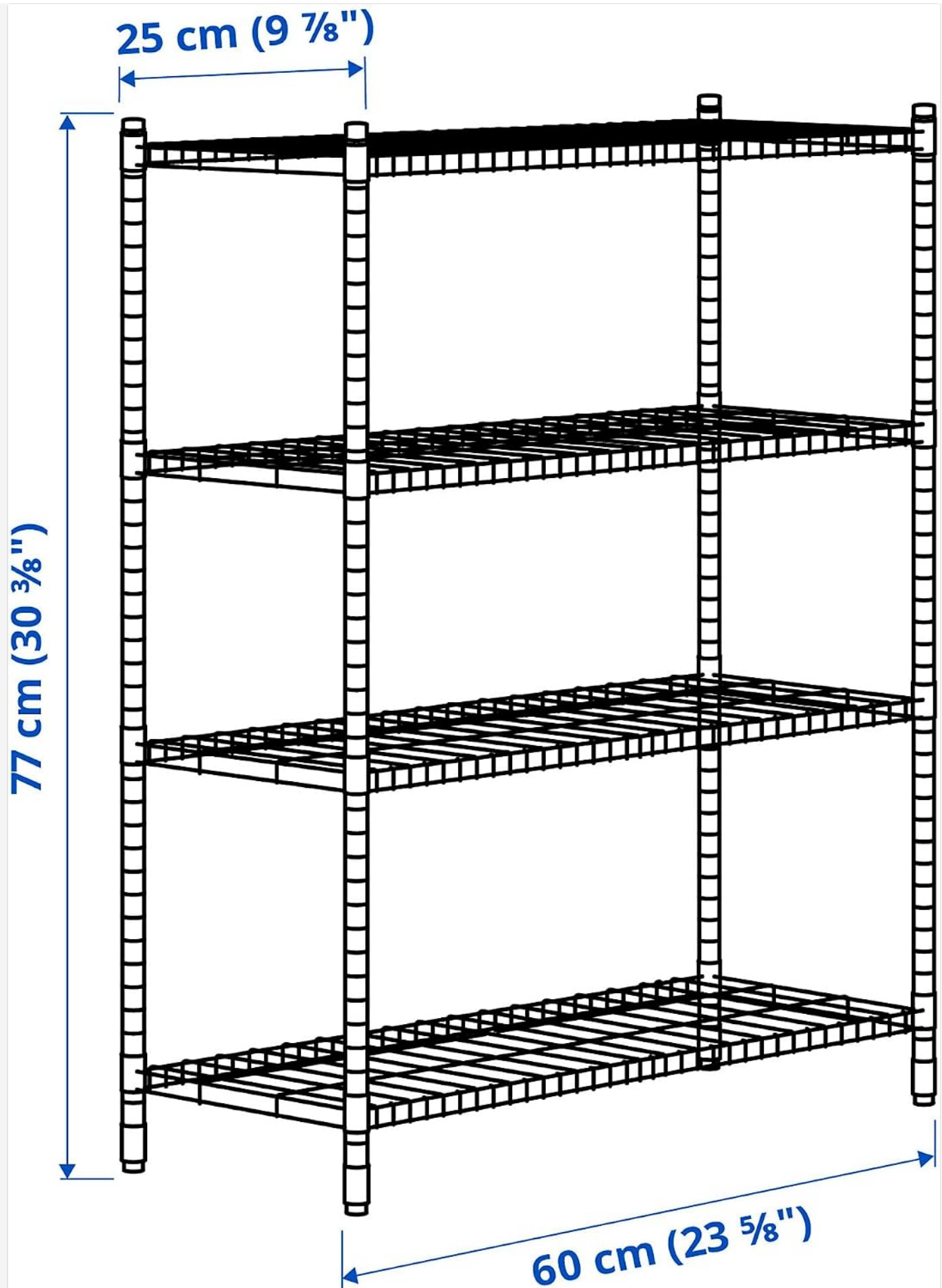
Figure 5: A dimensional diagram of an OMAR shelf unit, illustrating typical measurements within the series.
