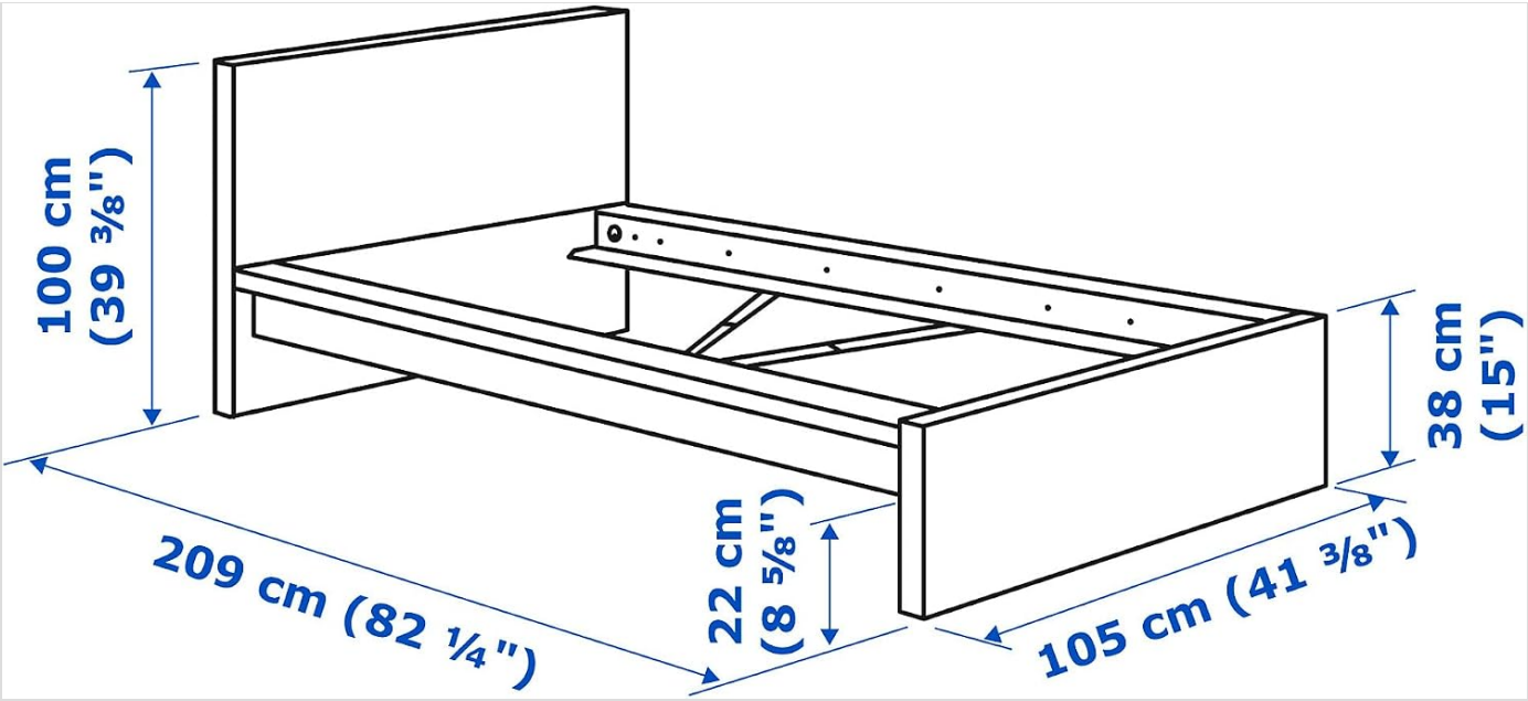
Image: Dimensional diagram of the MALM bed frame, showing height, length, and width.
