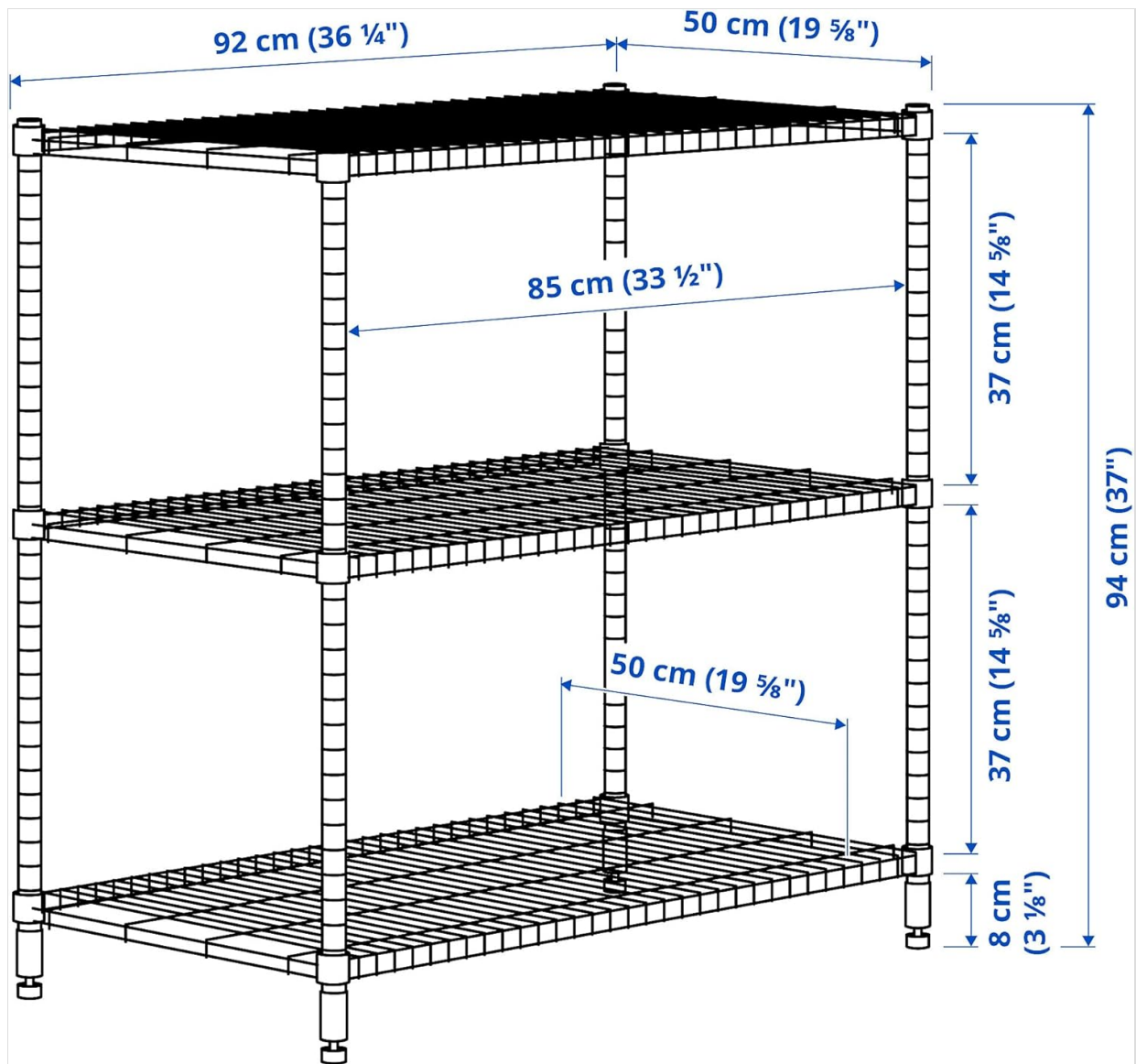
Figure 4.2: Dimensional drawing providing key measurements for the shelf, including overall height, width, depth, and shelf spacing.
