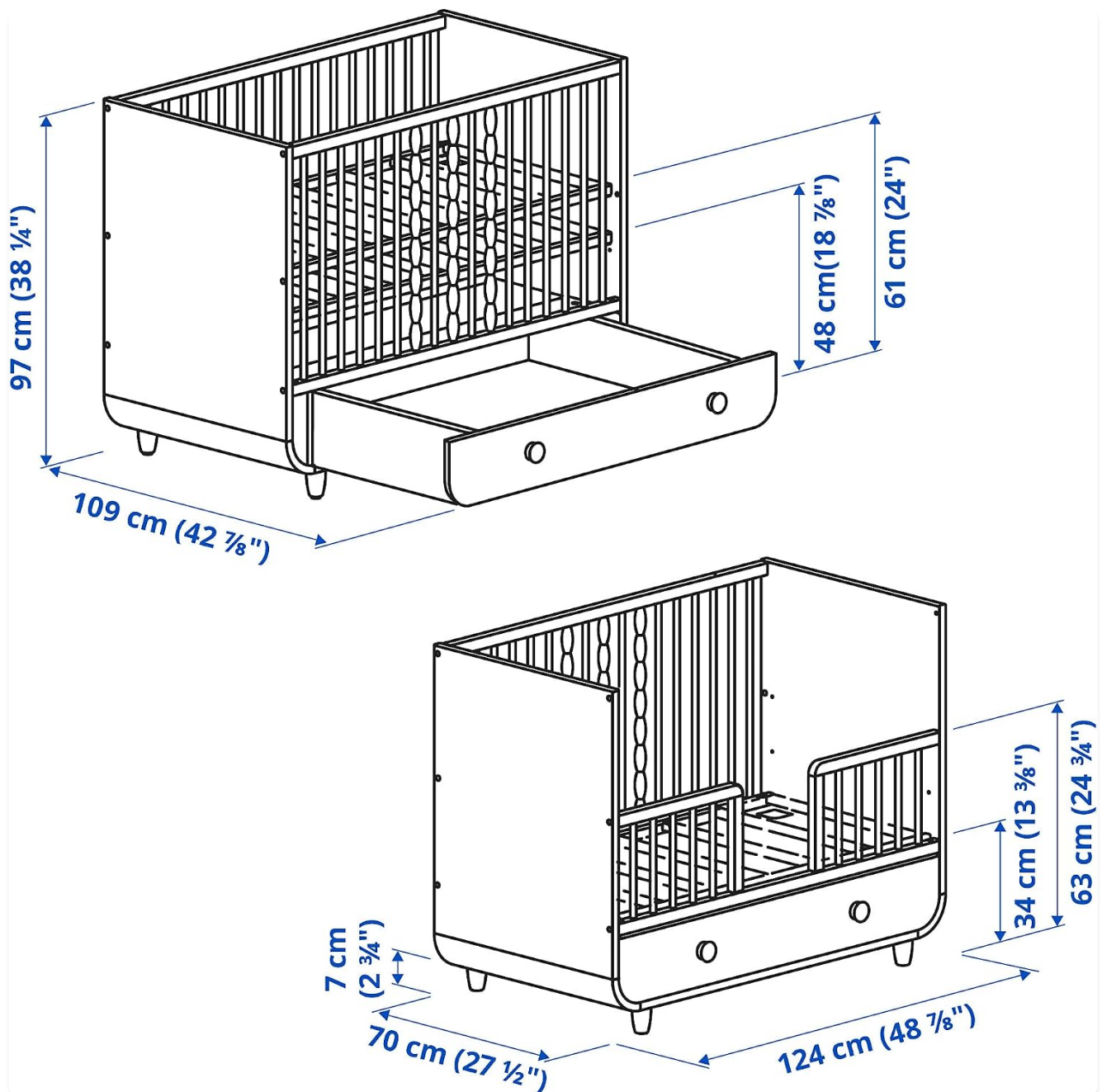
Image: Detailed dimensional diagram illustrating the various measurements of the Myllra crib, including overall dimensions and drawer size.
