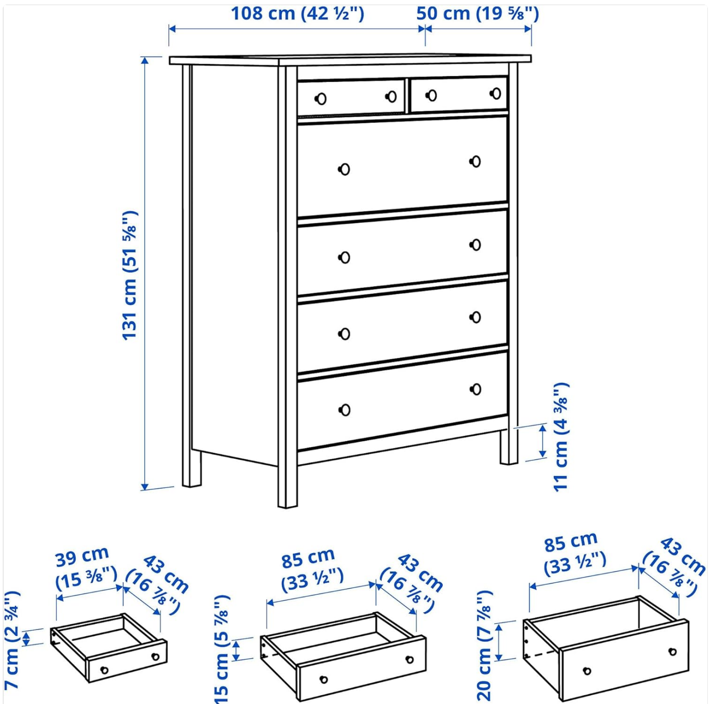
Figure 3: Detailed dimensions of the HEMNES chest and its various drawer sizes, crucial for planning placement and understanding capacity.
