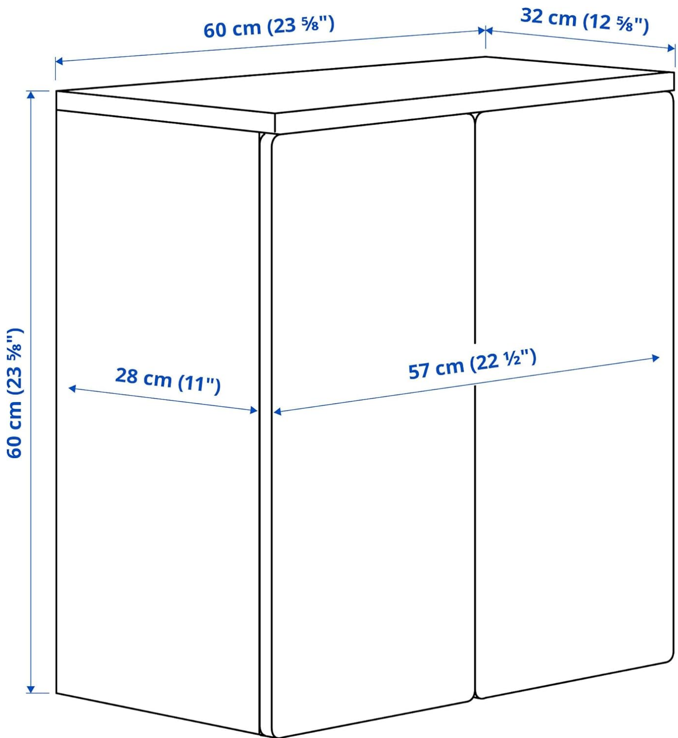
Figure 6: Dimensional diagram of the SMÅSTAD Wall Cabinet.
