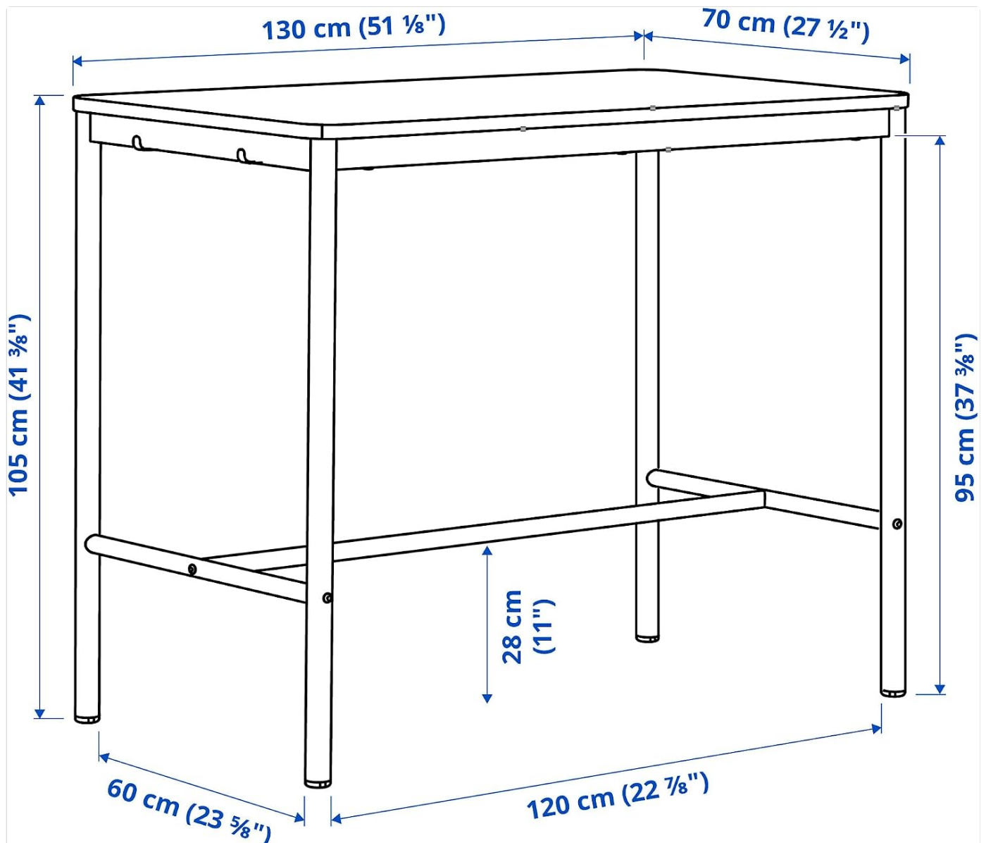
Figure 2: An illustration detailing the dimensions and structural components of the TOMMARYD table, useful for assembly reference.
