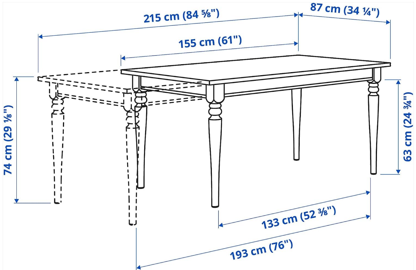
Image: Diagram illustrating the dimensions of the IKEA INGATORP table in both compact and extended states. Length: 155 cm (compact) / 215 cm (extended), Width: 87 cm, Height: 74 cm.
