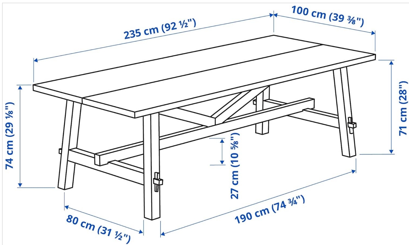
Image: A technical diagram illustrating the dimensions of the SKOGSTA Dining Table, including length, width, and height.
