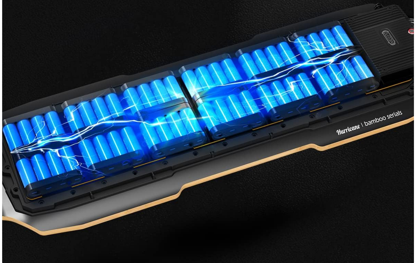
Figure 3: Internal view of the 725.8Wh 12S4P Molicel P42A Battery pack, showing its robust cell arrangement.
