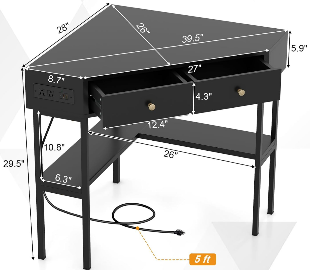
Figure 3.1: Detailed dimensions of the corner desk, including tabletop width, depth, and height, as well as drawer and shelf measurements.
