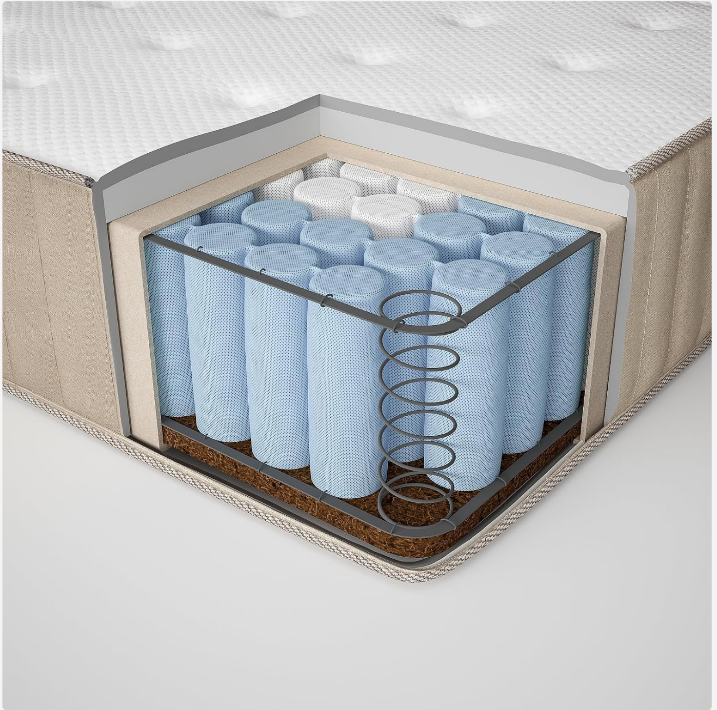
Figure 3: An internal view of the VATNESTRÖM mattress, highlighting the individually wrapped pocket springs and natural material layers.
