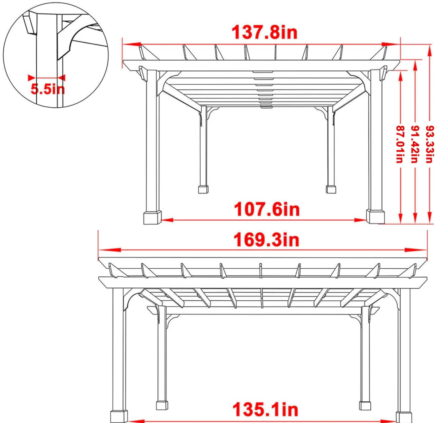
Image 4.1: Dimensional drawing of the pergola, including post size and overall measurements.
